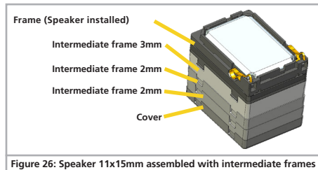
Figure 26: Speaker 11x15mm assembled with intermediate frames
