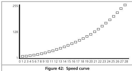
Figure 42: Speed curve
