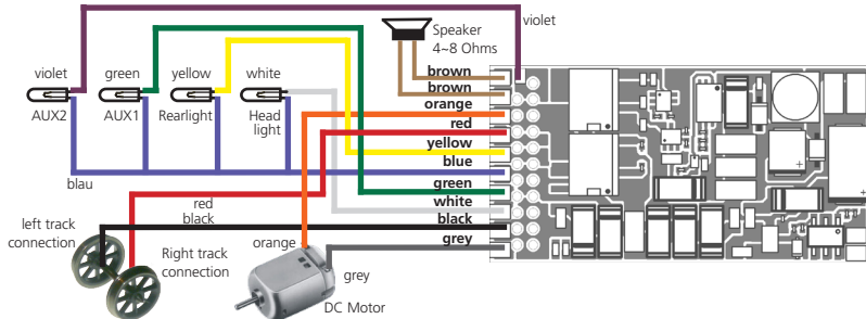
Figure 17: Wiring diagram for LokSound 5 (Wiring example)
